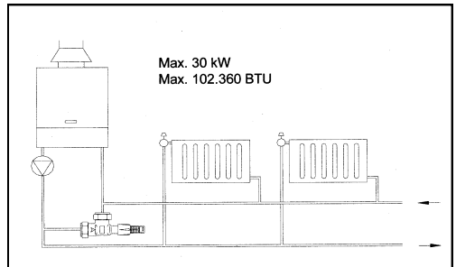
Fig.1 Installation example
